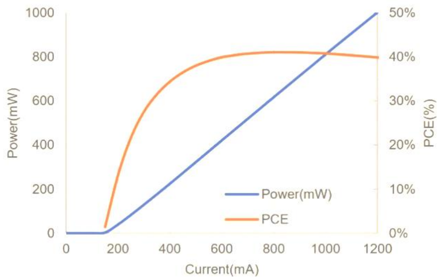
Typical LI Curve
