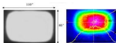
Beam angle: 110°x85°
