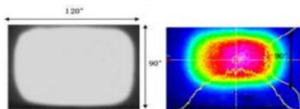
Beam angle: 120°x90°
