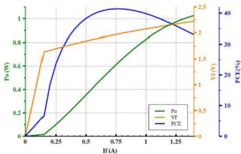
LIV Graph
