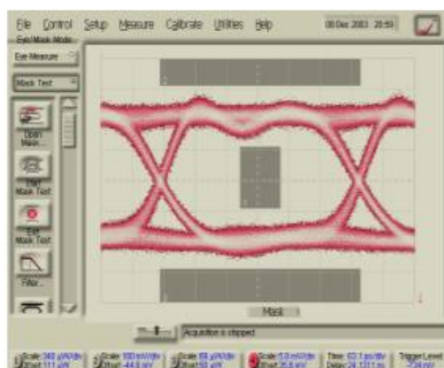
Eye Diagram
