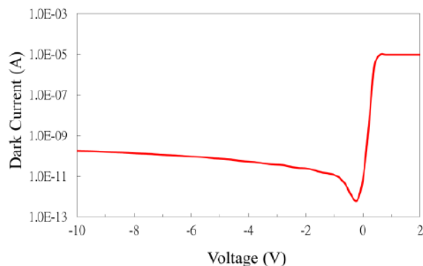
Fig. 1 Typical I-V Curve
