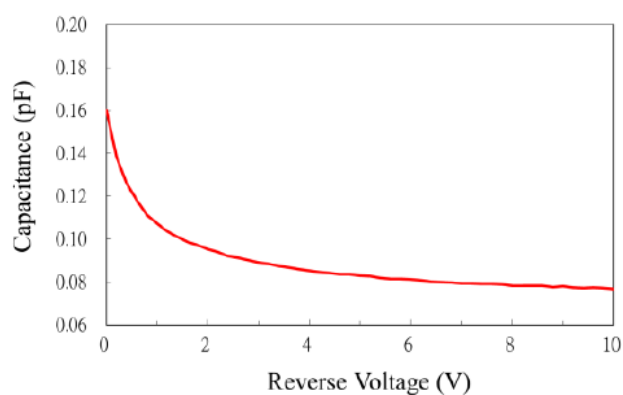
Fig. 2 Typical C-V Curve
