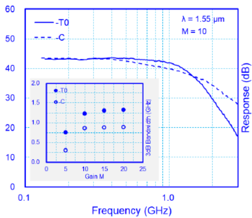
Frequency Response
