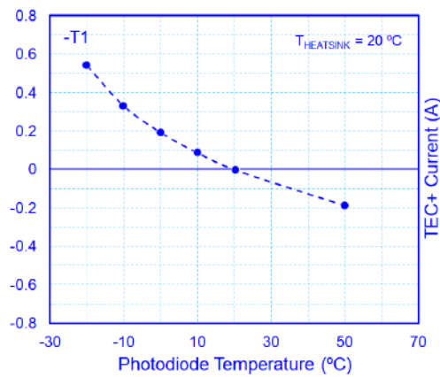
TEC Performance
