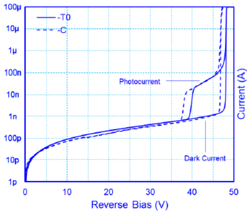
Dark / Photo-Current
