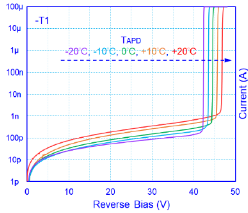
Dark Current
