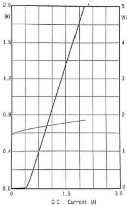
P-I-V CURVE
