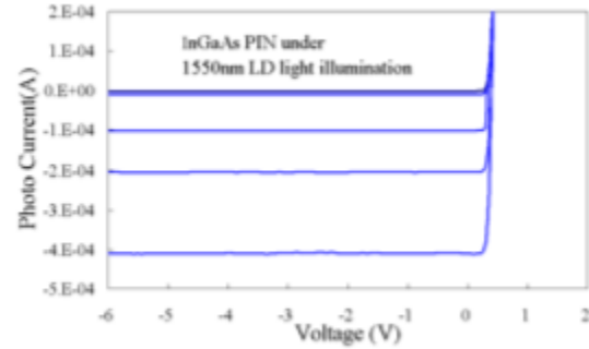
Fig. 2 Typical Photo-Current
