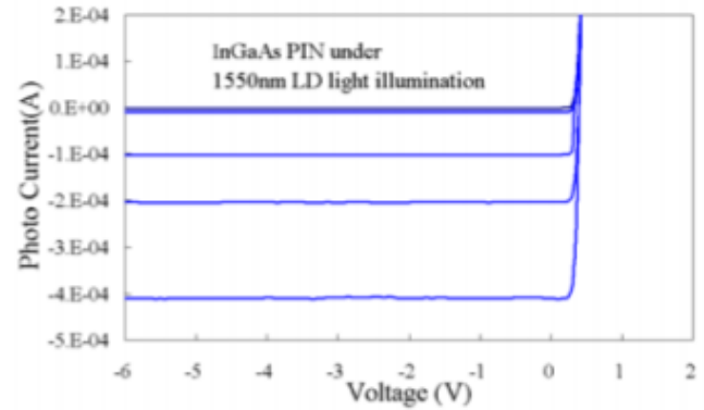
Fig. 2 Typical Photo-Current
