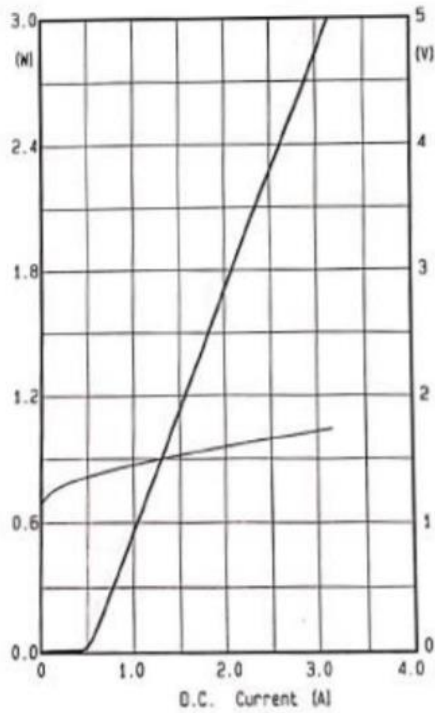
P-I-V CURVE
