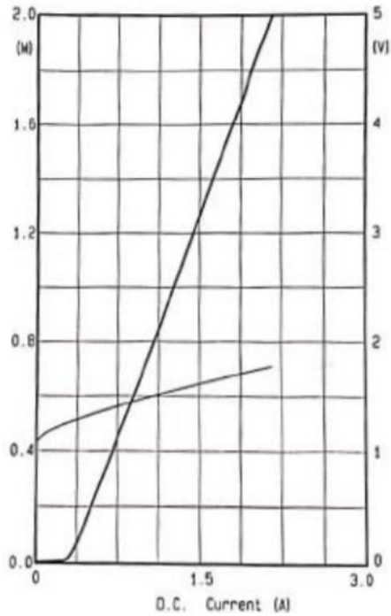
P-I-V CURVE
