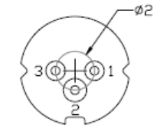
PIN CONFIGURATION
