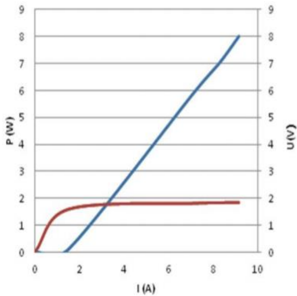
P-I-V CURVE
