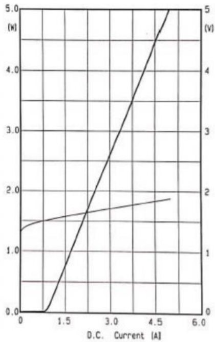
P-I-V CURVE
