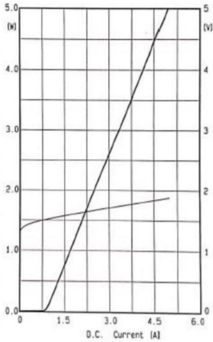
P-I-V CURVE
