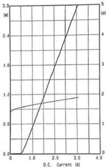
P-I-V CURVE
