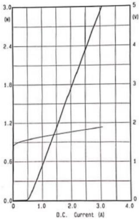
P-I-V CURVE
