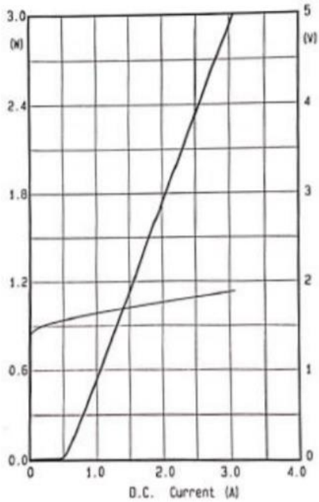
P-I-V CURVE
