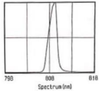
SPECTRAL CURVE
