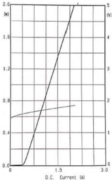
P-I-V CURVE
