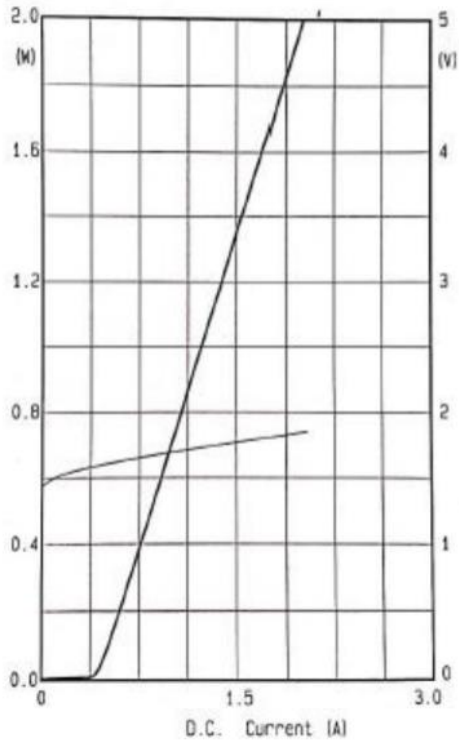
P-I-V CURVE
