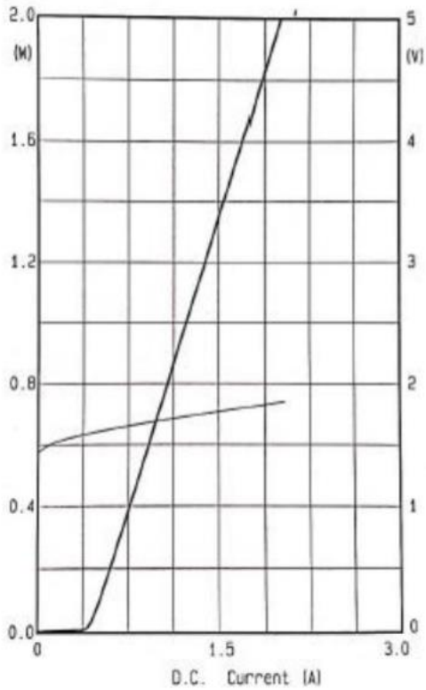
P-I-V CURVE
