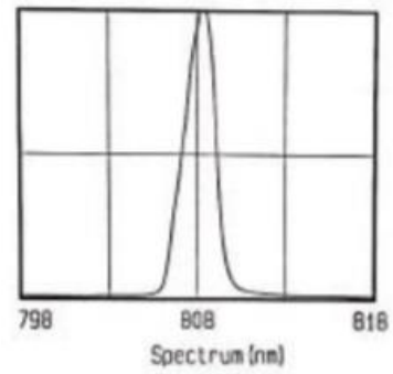
SPECTRAL CURVE
