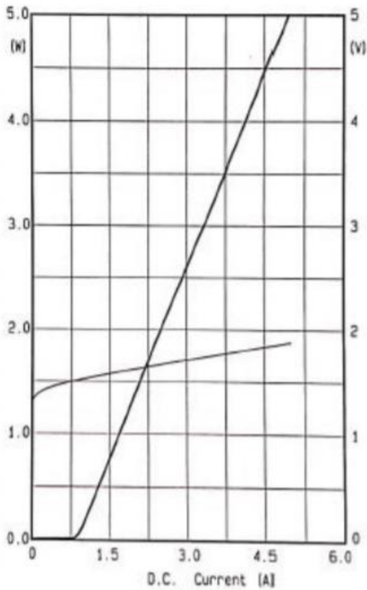
P-I-V CURVE
