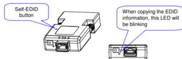
Figure 2 – Self-EDID Mode
