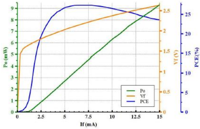
LIV Graph
