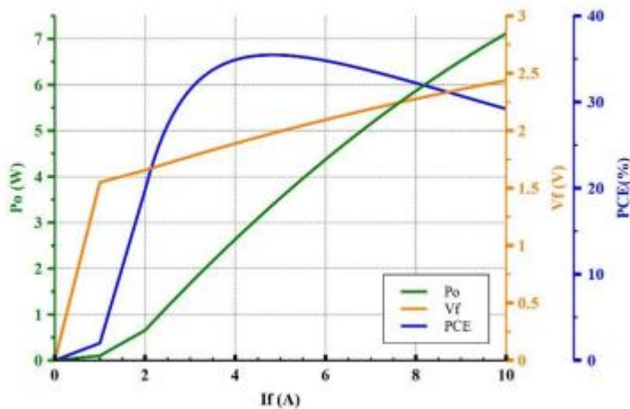
LIV Graph
