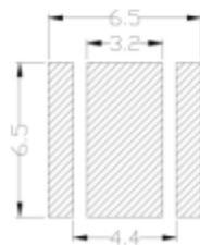
Recommend Solder Pad (mm)
