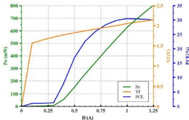
LIV Graph at 25°C
