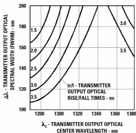
Figure 1 – LED Spectral Width
